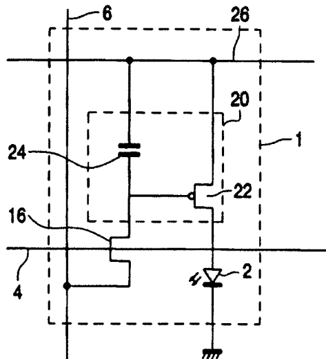
FIG. 2 PRIOR ART
